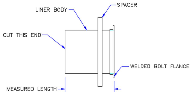
Figure 3: Cut the Liner Body to the measured length between adjacent sections.
