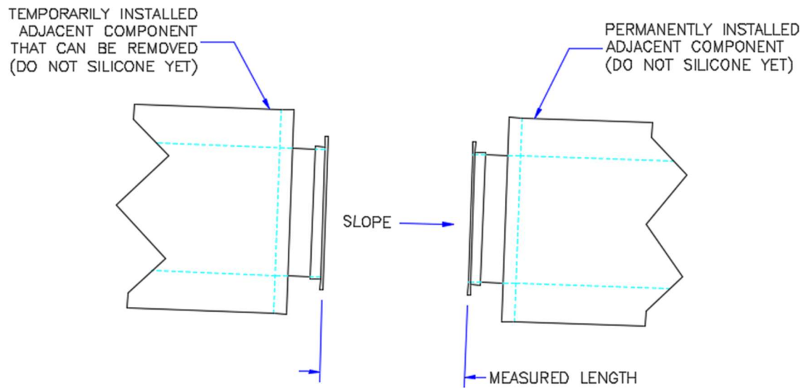
Figure 2: Measure the length between the two adjacent components.
